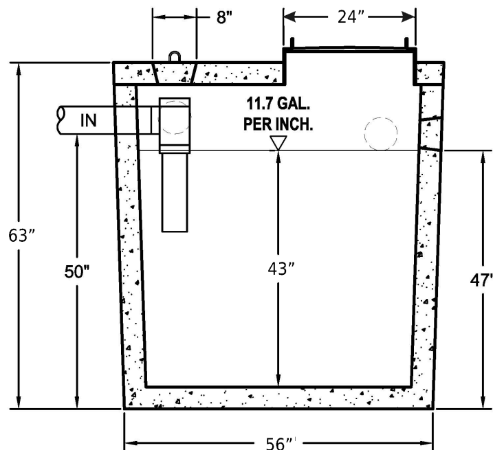
SECTION VIEW
