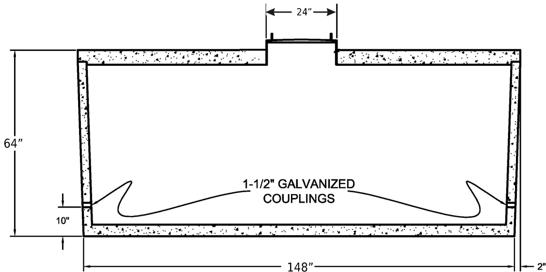
SECTION VIEW
